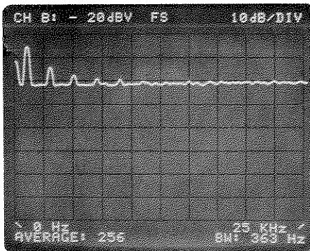
RMS average
