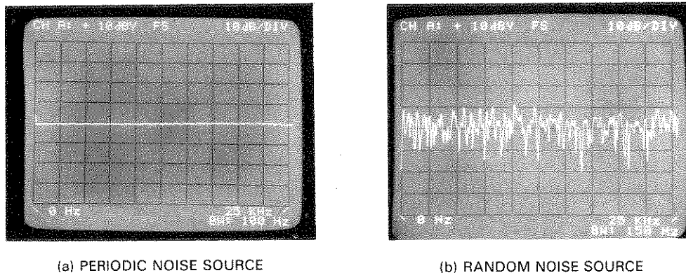
Figure 3-10. Noise Source Spectrums.
