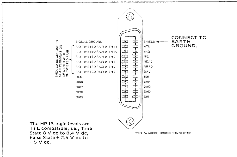
Figure 3. HP-IB Connector.
