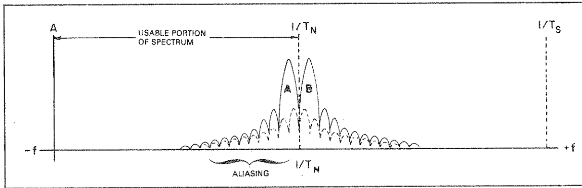
Figure 3-36. Aliasing.
