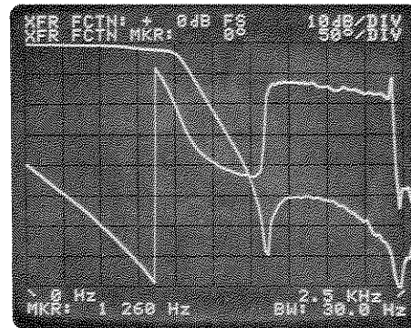
filter analysis
