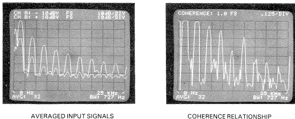
Figure 3-23. The Coherence Relationship Between Two Signals.
